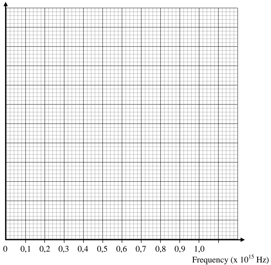
Max. E_K of photoelectrons against Frequency of Radiation
